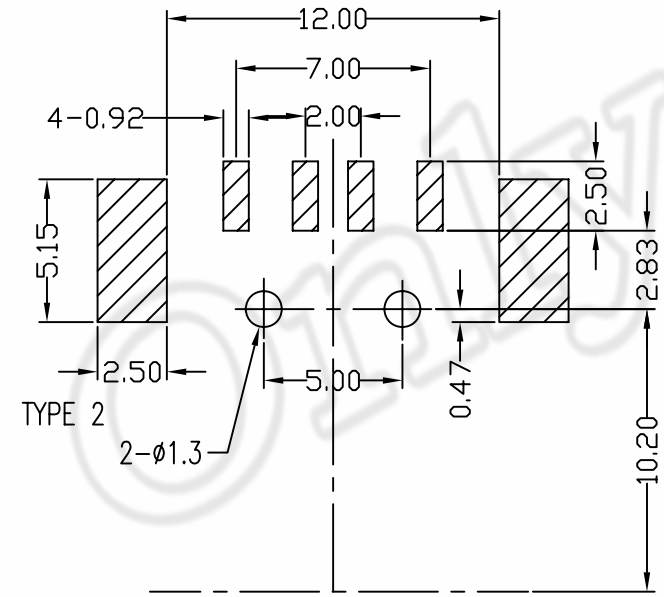
PCB LAYOUT
